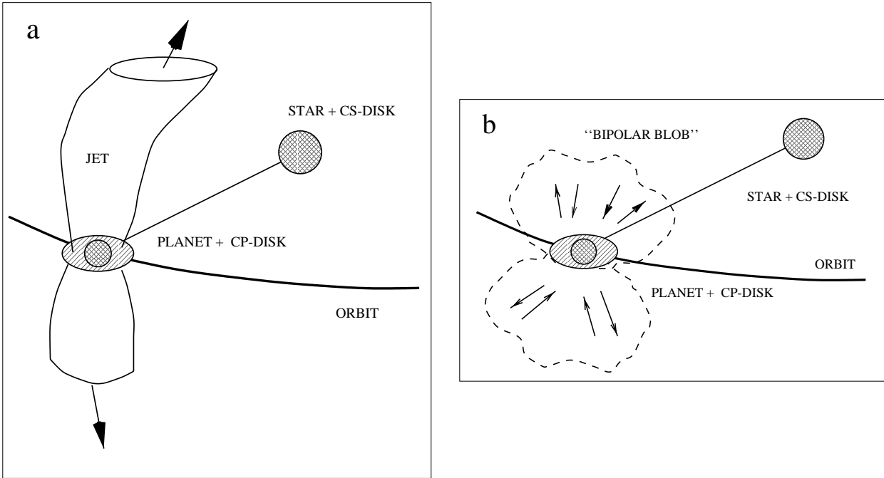
Fig. 1. Model scenario of hypothetical outflows from circum-planetary accretion disks. A protoplanet surrounded by a circum-planetary disk (“CP-disk”) is located within the circum-stellar disk (“CS-disk”). Depending on the outflow velocity achieved, two different types of outflow activity are possible – a large scale outflow ( a ), possibly collimated, or a bipolar blob ( b ) orbiting with the planet.
