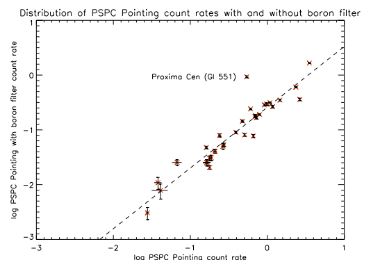
Figure 6. Comparison of X-ray count rates for stars detected in the PSPC pointing program with and without the boron filter.
