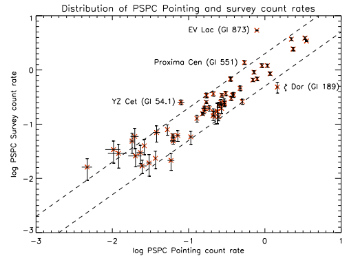
Figure 4. Comparison of X-ray count rates for stars detected both in the all-sky survey and the PSPC pointing program. The dashed lines indicate a variation of a factor of 2 from unity. Stars with large deviations are labeled, they are all known flare stars.
