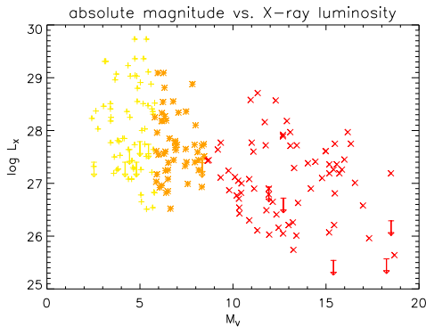
Figure 2. X-ray luminosity as function of absolute magnitude for the three samples. The range in X-ray luminosity is about three orders of magnitude independent of spectral type while the median X-ray luminosity is decreasing with increasing M_V .
