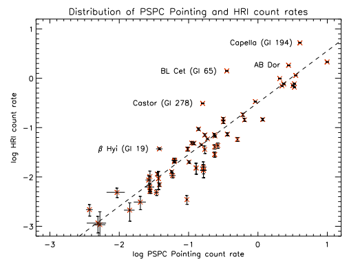
Figure 5. Comparison of X-ray count rates for stars detected both in the PSPC and HRI pointing program.
