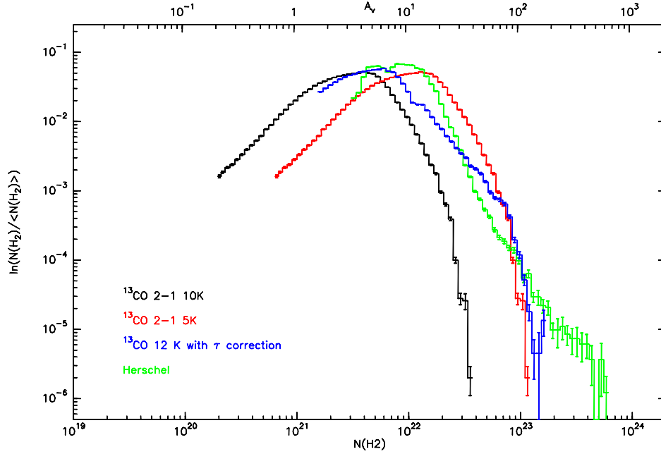
Fig. 13. Probability distribution functions of the \text{H}_2 column density derived for the whole W43 complex from different data sets and methods. The y -axis is normalized to the mean value of N(\text{H}_2) . Isothermal CO column densities (5 and 10 K) are plotted in red and black; CO derived values with optical depth correction are in blue, and Herschel results are in green.
